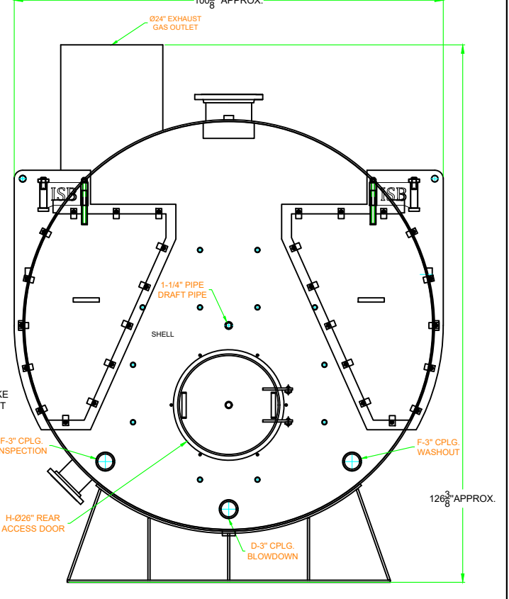
REAR VIEW
