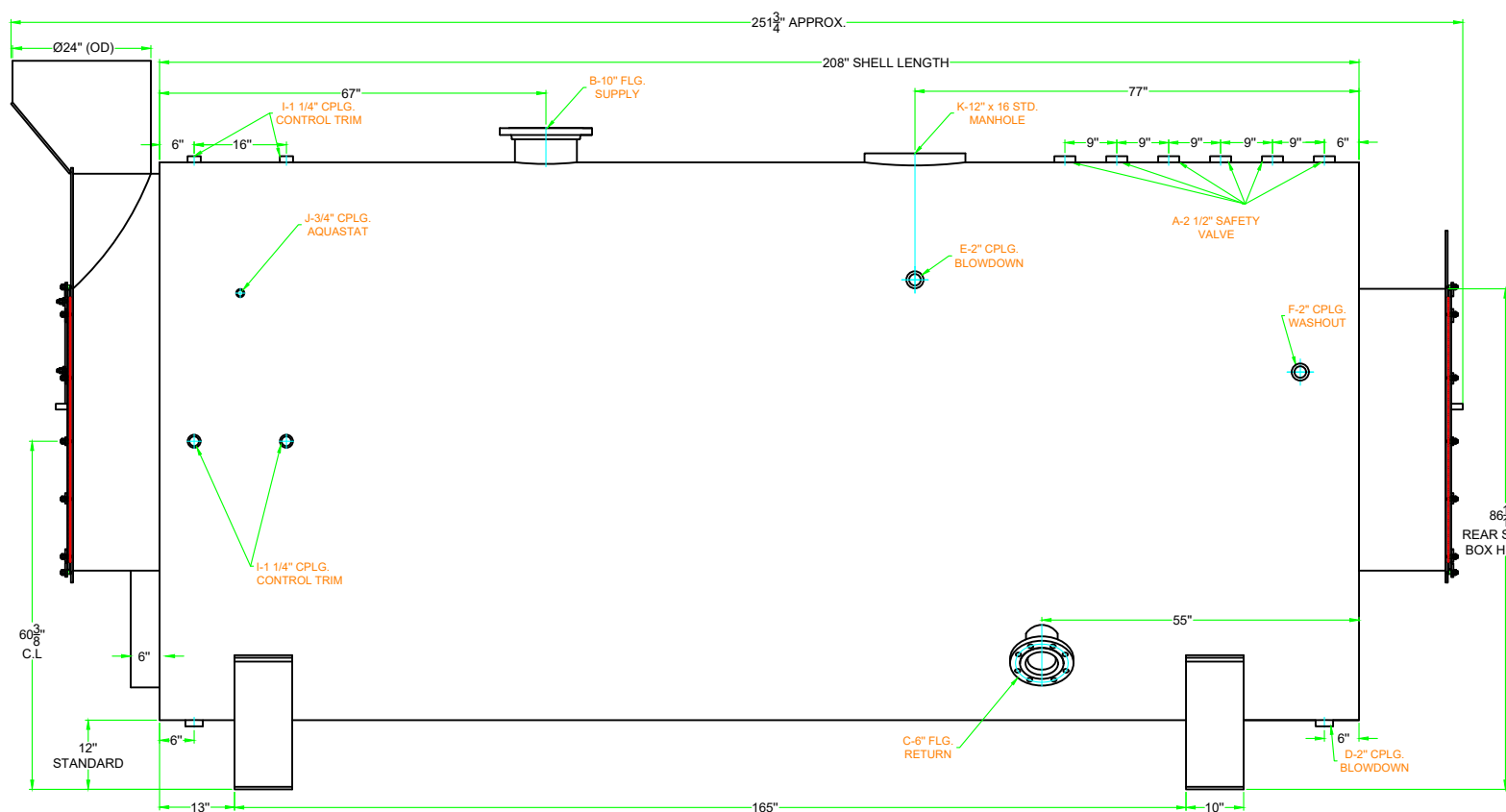
SIDE VIEW
