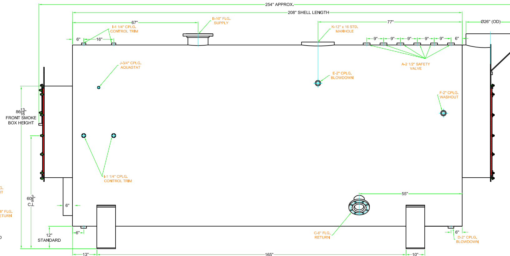
SIDE VIEW
