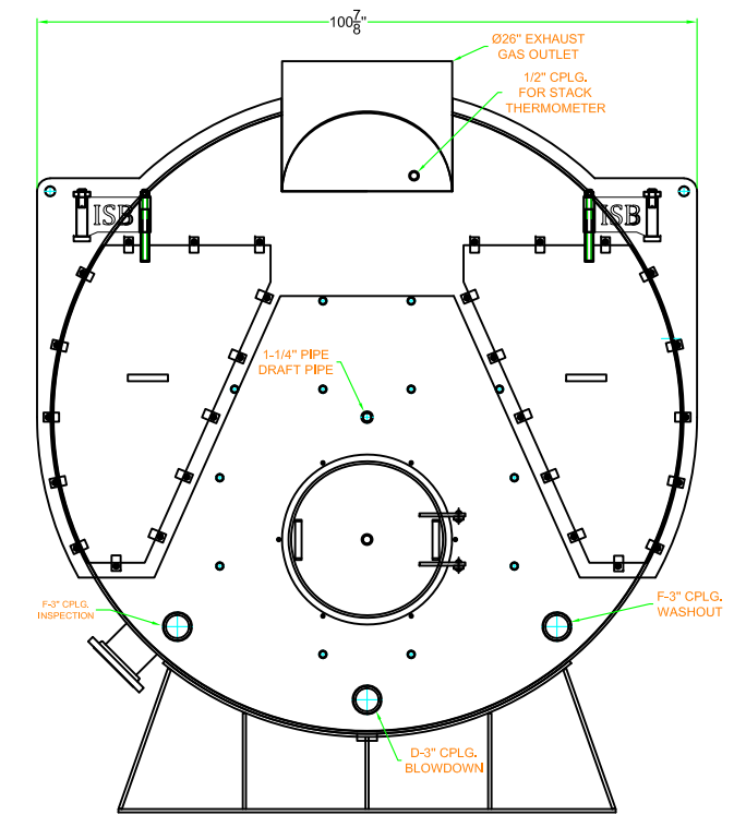
REAR VIEW
