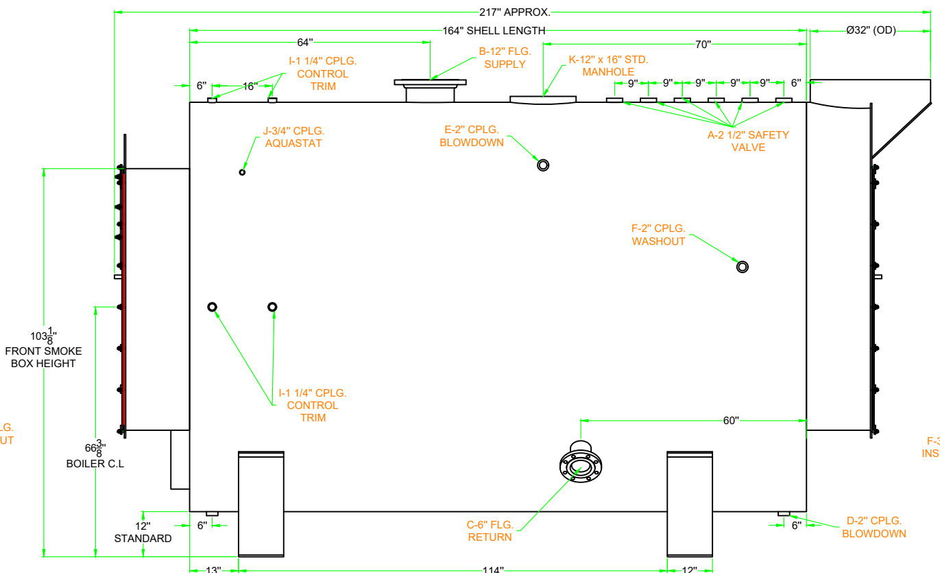
SIDE VIEW
