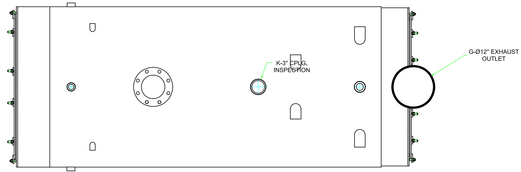
TOP VIEW
