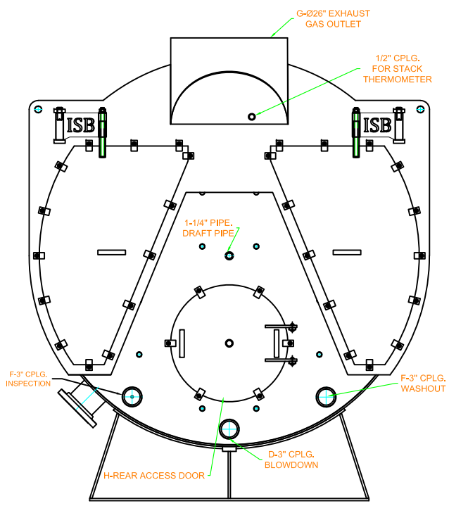
REAR VIEW
