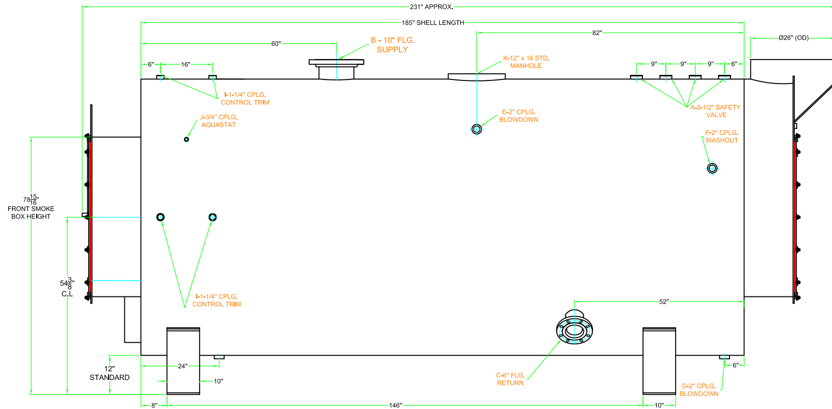
SIDE VIEW
