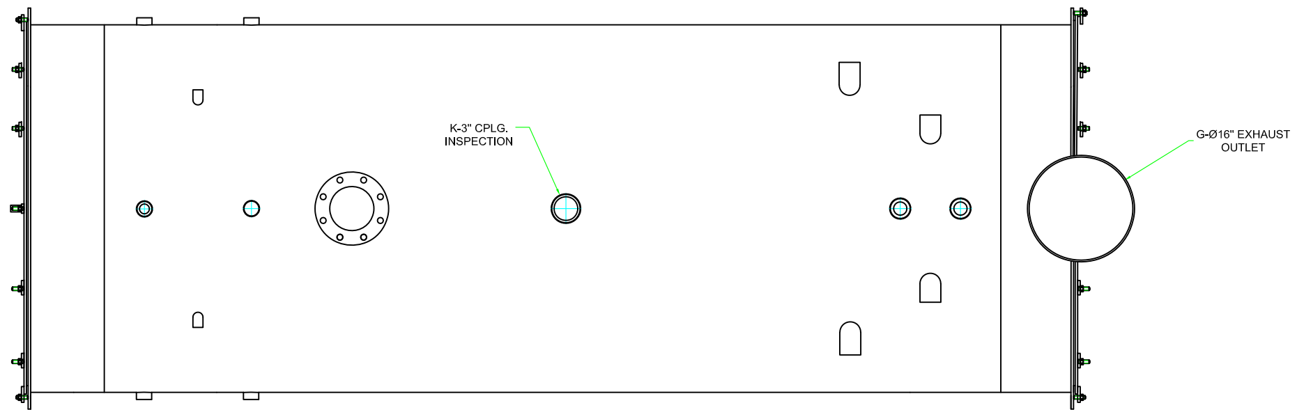
TOP VIEW
